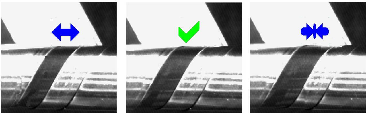
Tape Proces Regulator. Turning to 1800rpm measures and adjusts the speed.
